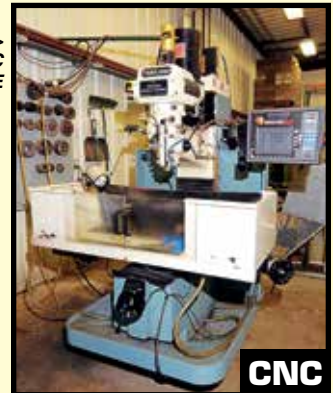
TRAK MDL. DPM2 3-AXIS CNC VERTICAL MILLING MACHINE
