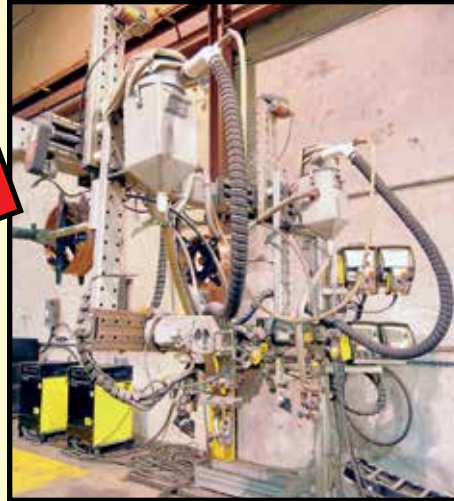
CLOSE-UP OF ESAB MECH-TRAC WELDING HEADS
