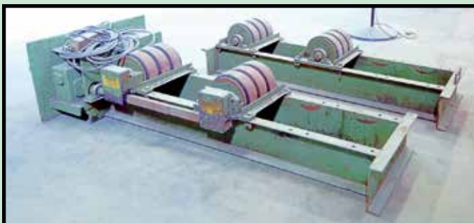
20 T. JOE FULLER POWER TURNING ROLL SETS
