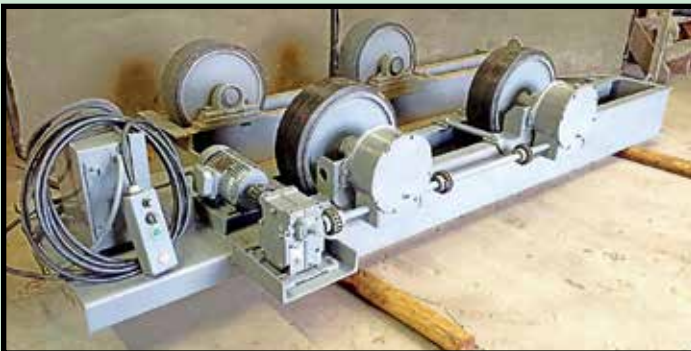
RANSOME 30 T. POWER AND IDLER SET
