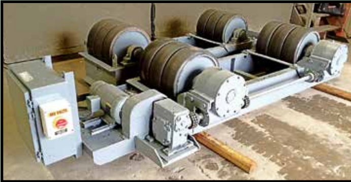
RANSOME 90 T. POWER AND IDLER SET
