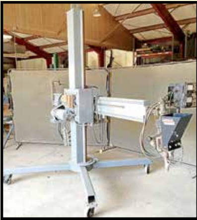
ARONSON 6 X 6 WELDING MANIPULATOR
