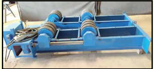
WELD WIRE 20 T. CAP. TANK TURNING ROLL SET
